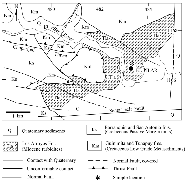
Figure 3. Geologic map of the El Pilar area with sample location of Los Arroyos Formation [25].
