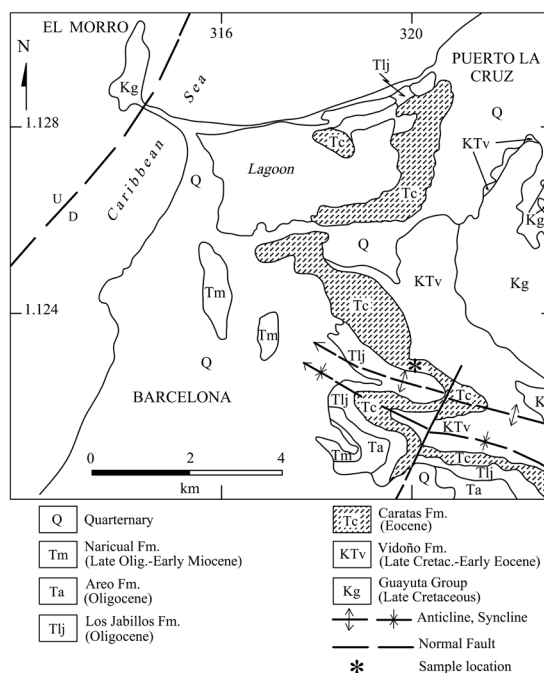
Figure 2. Geologic map of Barcelona-Puerto La Cruz area showing the location of Caratas Formation sample. UTM Coordinates zone 20 ( \times 10^{-3} ) datum La Canoa. After Keller [12].
