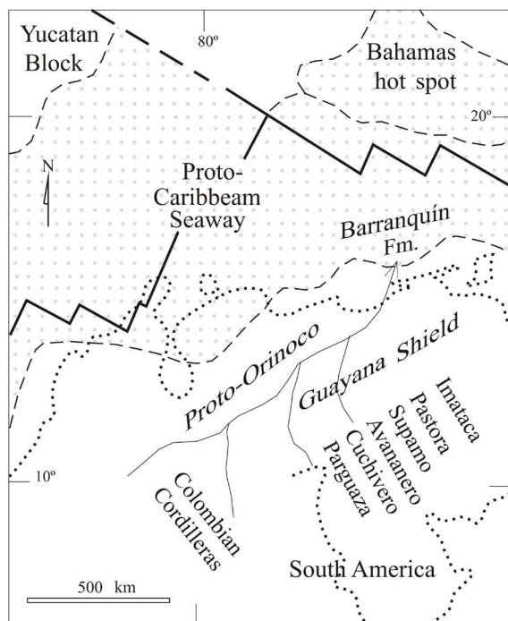
Figure 7. Paleogeography and global tectonic configuration for Early Cretaceous. The Barranquín Formation and the sediments of the Güinimita and Tunapuy formations were deposited in the passive margin of northern South America. Present day coastline is depicted for reference purposes only. Base map after Pindell et al. [27], proto-Orinoco after Noguera et al. [20].
