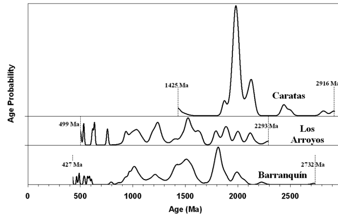
Figure 4. Probability density plot of U-Pb detrital zircon ages from Caratas (n=46) and Los Arroyos (n=47) formations. Barranquín Formation (n=189) data from Noguera et al. [20].
