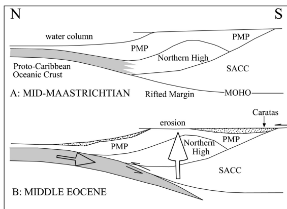
Figure 6. Geodynamic model of Pindell et al. [8] during Mid-Maastrichtian (A) and Middle Eocene (B) showing the position of the Caratas basin receiving sediments only from the Guayana Shield. PMP: Passive margin prism. SACC: South American Continental Crust.
