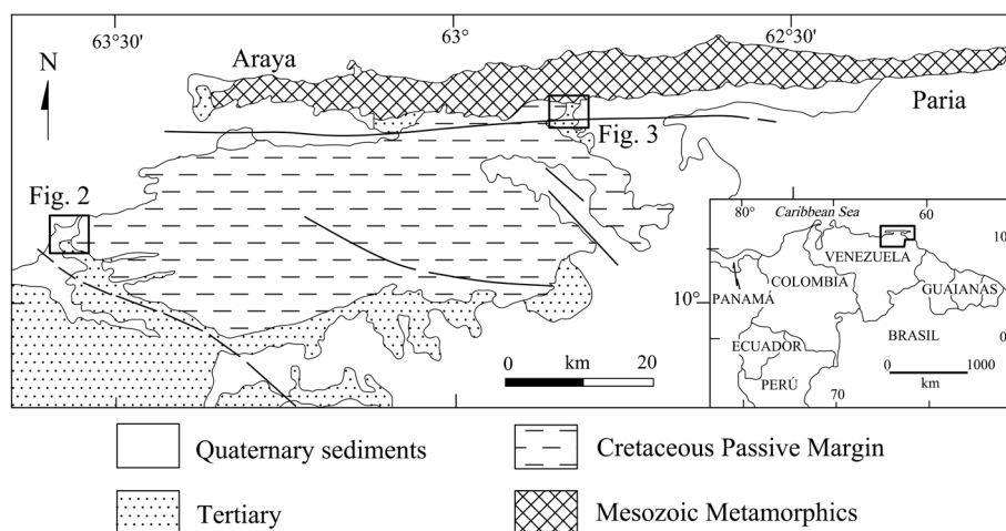
Figure 1. Geologic map of northeastern Venezuela with rectangles showing the location of further detailed figures. Simplified after [9].
