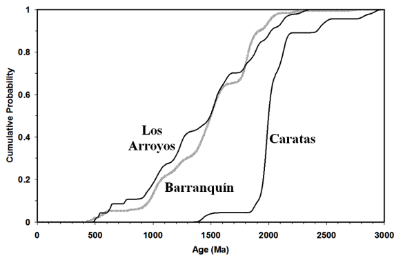
Figure 5. Cumulative Probability Density Plot of U-Pb zircon detrital zircon ages from Caratas, Los Arroyos and Barranquín formations.
