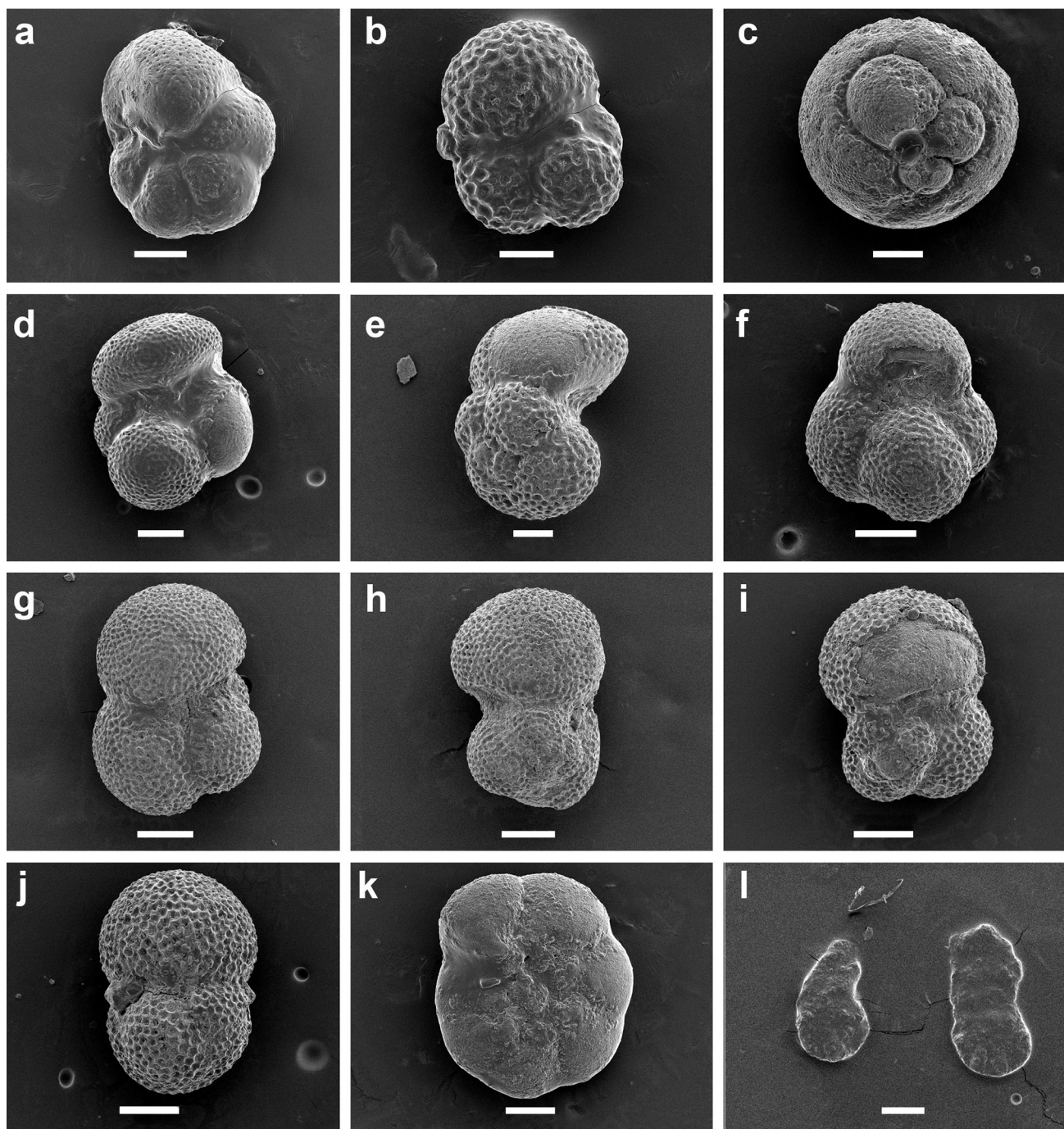
Fig. 4 Foraminifera recovered at Quebrada Corralito. (a–k, sample S3; l, sample S4). a Globorotalia archaeomenardi BOLLI; b , Globigerina praebullooides BLOW; c , Praeorbulina glomerosa (BLOW); d , e Globoquadrina dehiscens (CHAPMAN, PARR & COLLINS), apertural and side view; f Globigerinoides obliquus obliquus BOLLI; g ,
