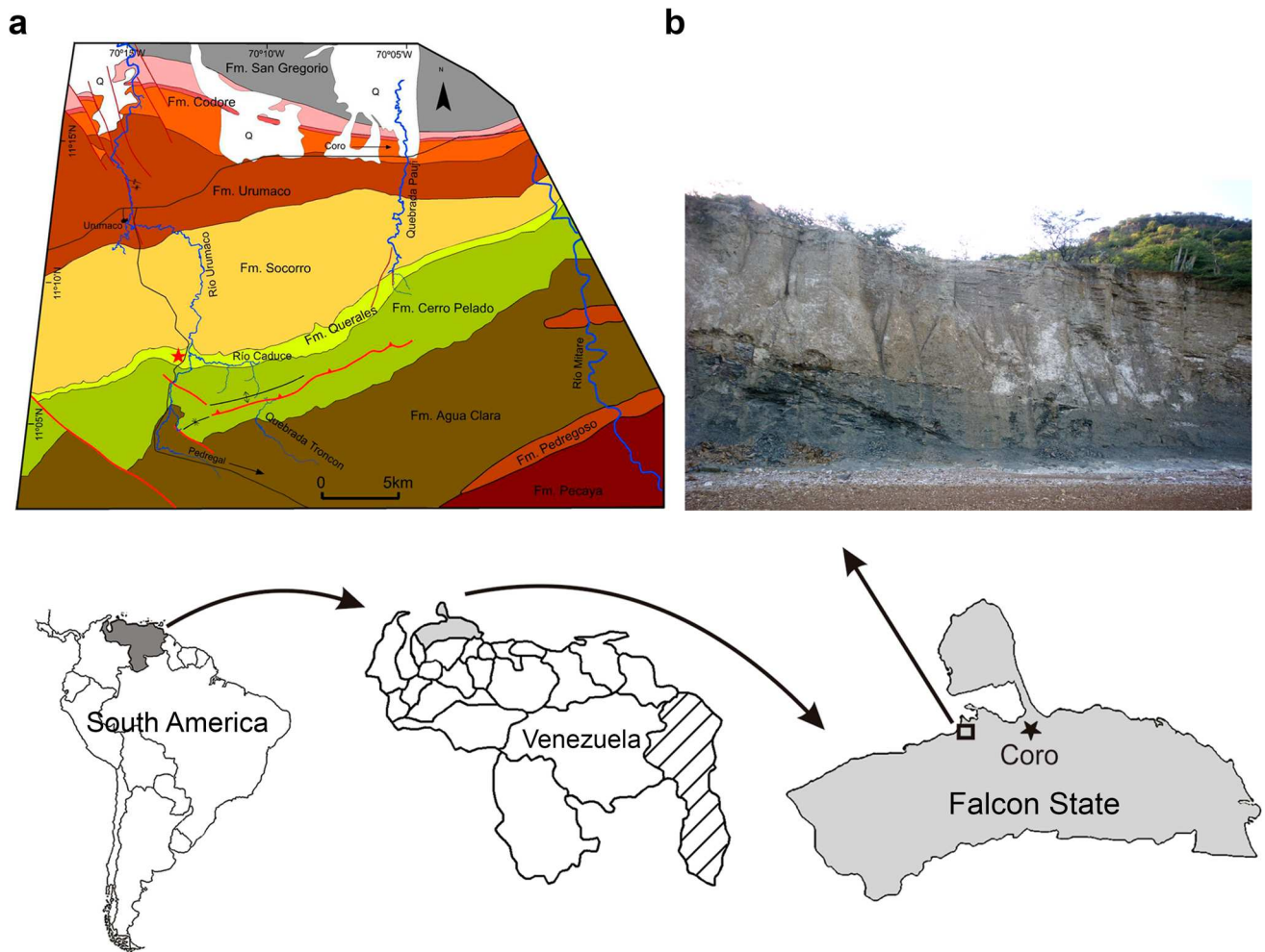
Fig. 1 a Geographical setting of “Quebraza Corralito” (QC) quarry of the Querales Formation, Falcon Basin, northwestern Venezuela. Examined site is indicated with a star ; GPS 11°07.180 N–
