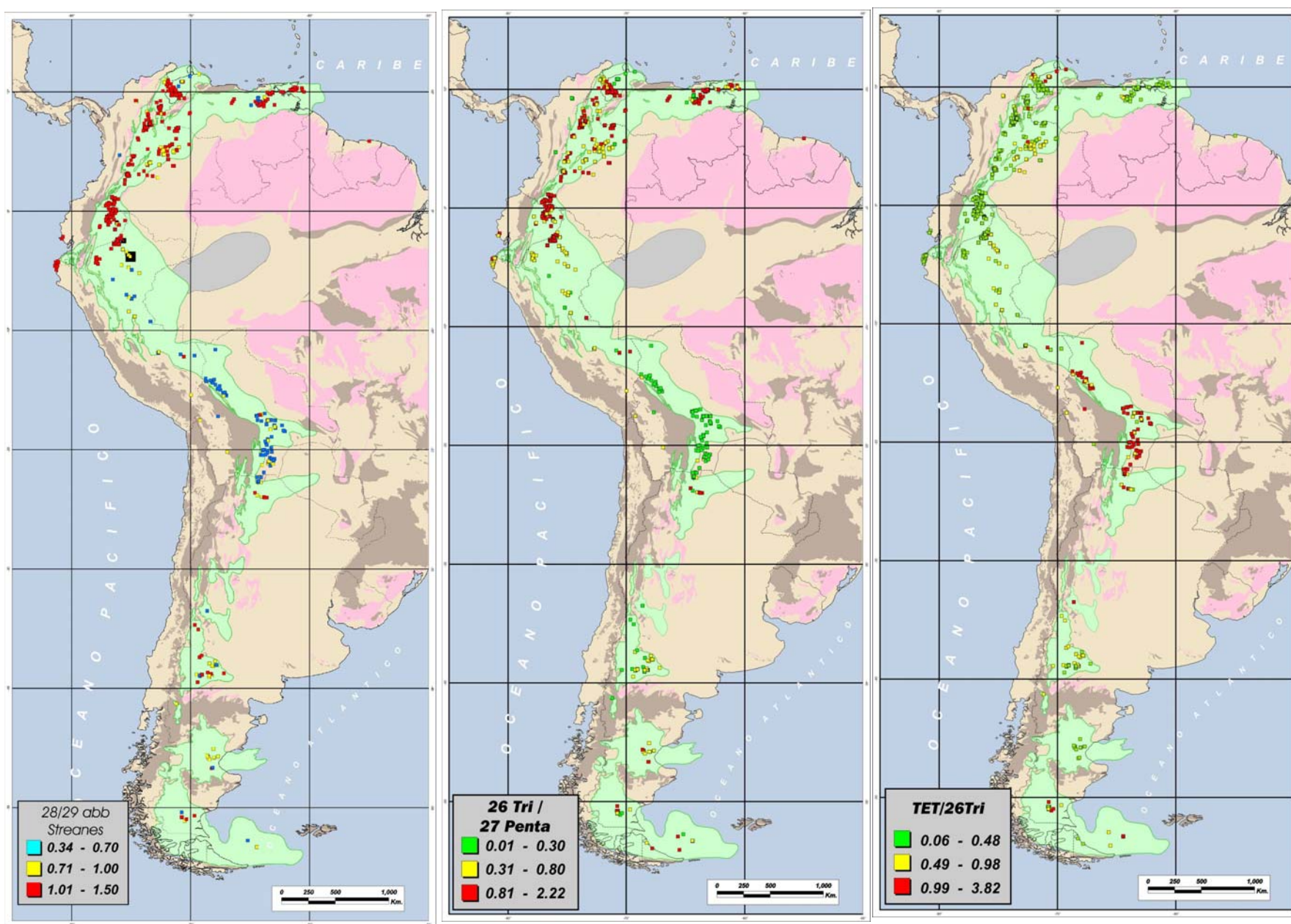
Figure 3. Variation of key biomarker parameters that vary as a function of lithofacies ( C_{24} tetracyclic terpane/ C_{26} tricyclic terpanes; values increase with increasing clastic input), anoxic conditions. ( C_{26} tricyclic/ C_{27} pentacyclic terpanes; values increase with anoxicity), and source age ( C_{28}/C_{29} \alpha\beta sterane ratio; for oils derived from marine shales, values typically decrease with source age).
