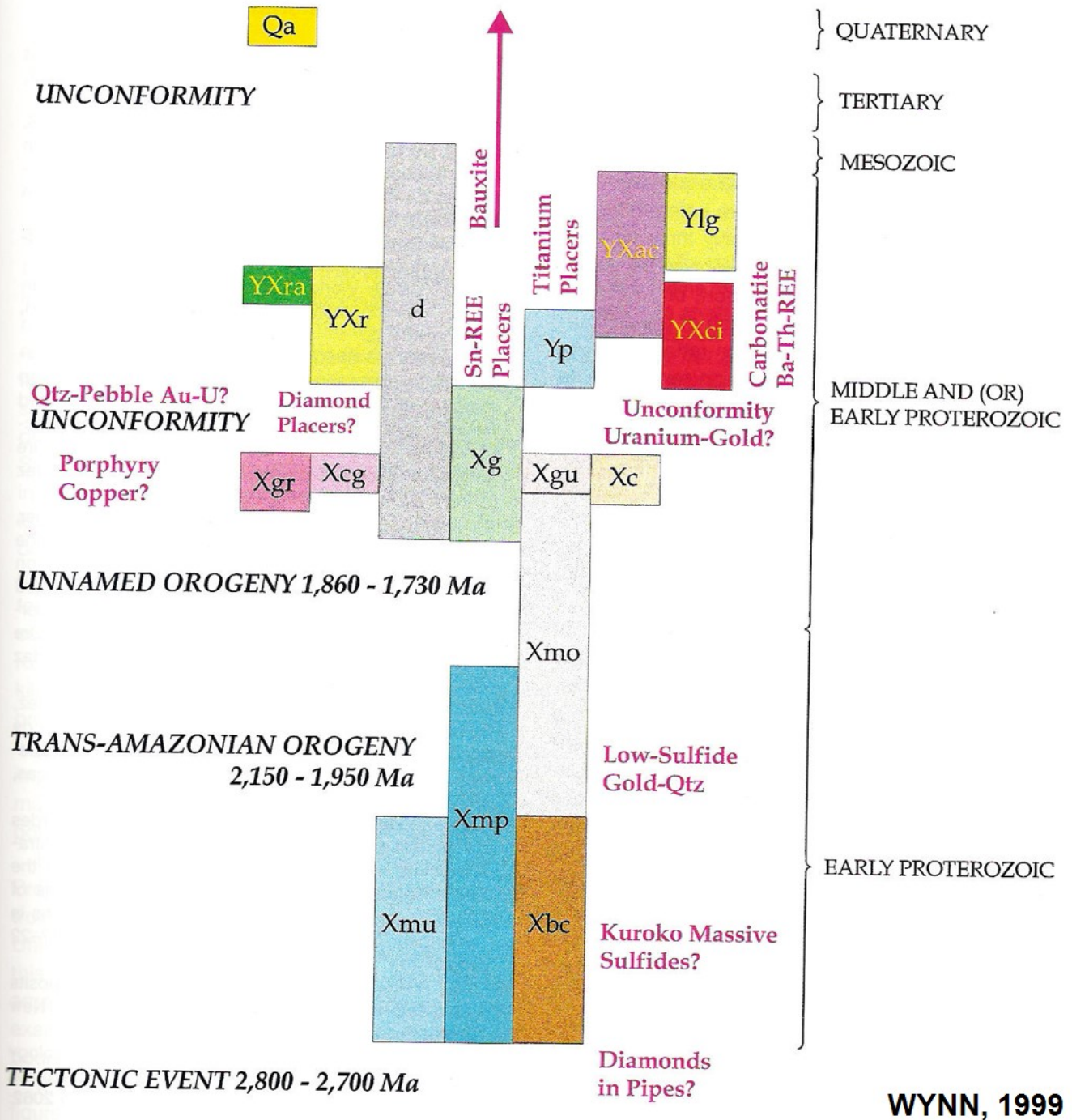
Fig. 3. Geologic correlation chart for the southwestern Venezuelan Guayana Shield, showing possible deposit models by geologic time.
