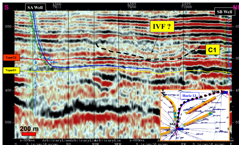
Fig 14: Seismic line along horizontal well Hor13 (black dotted trajectory) and using as reference vertical wells SA and SB. Between both vertical wells an anomaly in seismic response can be seen and interpreted as a possibly incised valley fill (IVF).
