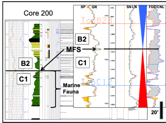
Fig 11: Core-log calibration for Well 200, showing the maximum flooding surface (MFS), ending the second transgressive system tract.
