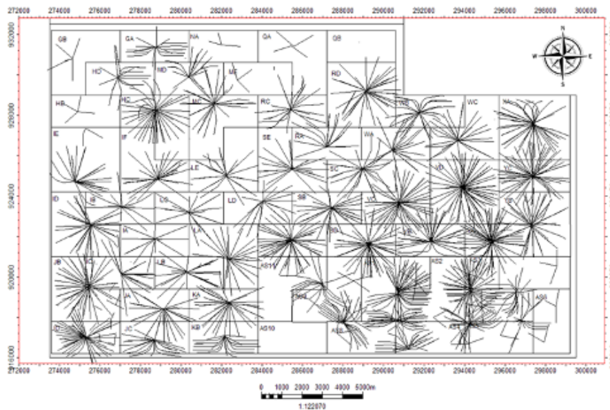
Fig 2: Study area, showing the cluster subdivision and the 2D projection of all horizontal wells drilled inside Oficina Formation. A radial pattern can be observed from the center of each cluster and a late pattern (fork type) in some clusters.
