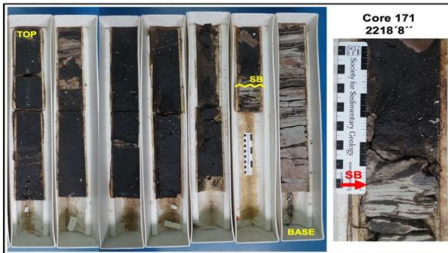
Fig 9: Core interval 2207'-2221' from well 171, where the interpreted new SB can be seen for C1 unit, with a sharp/erosive contact, and the sandy filling of the incision.
