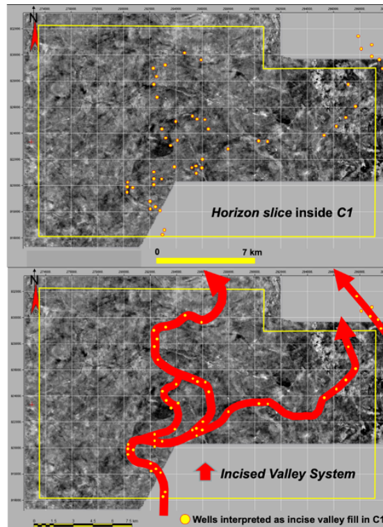
Fig 15: Time slice 50 milliseconds above base of unit C1 (uninterpreted above). 2D interpretation of the incised valley system for C1 unit (below) overlying the time slice. Notice the high sinuosity trajectory in some places, and its interpretation also outside the study area to the northeast. Yellow dots in both images, are wells interpreted as valley fill sediments.
