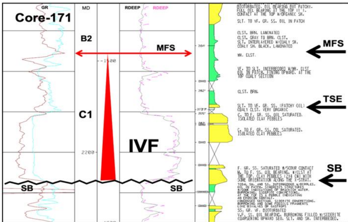
Fig 8: Well log and original core description (author unknow) of Core-171 showing the sedimentary section interpreted as an incised valley fill (IVF), within the C1 operational unit. Notice the interpreted SB at the base of the fluvial channel facies and the MFS upwards in the core section, coincident with at GR peak response (high radioactivity).
