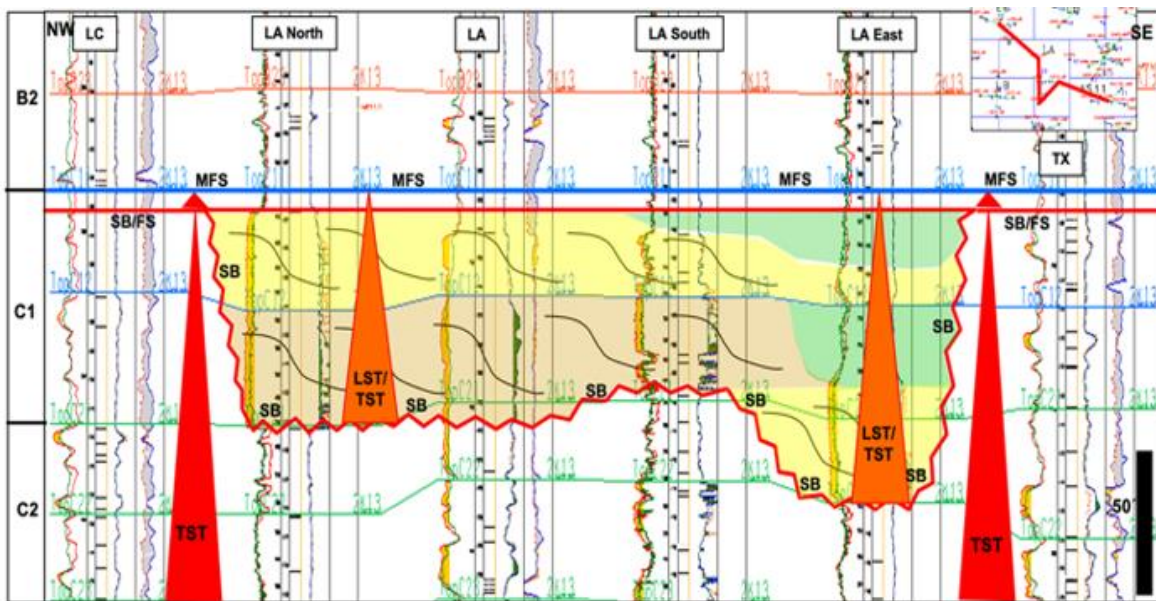
Fig 7: Sequence stratigraphy interpretation for clusters LC/LA/AS11, showing the presence of an interpreted incised valley, cutting the normal TST vertical pattern for C2/C1 units observed in wells LC and TX. The cross section spans about 6 km between both wells. The datum corresponds to the MFS at the top of C1 unit. (Green color = shaly fill, yellow/brown color = sandy fill).
