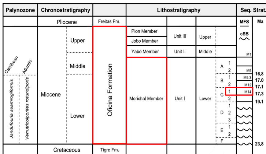
Fig 5: Stratigraphic column at Faja del Orinoco, and geological ages. Modified from [15].
