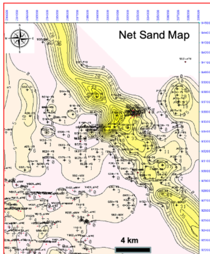
Fig 6: Net Sand Map from operational unit C1 at PetroAnzoategui field, northeast of the study area.
