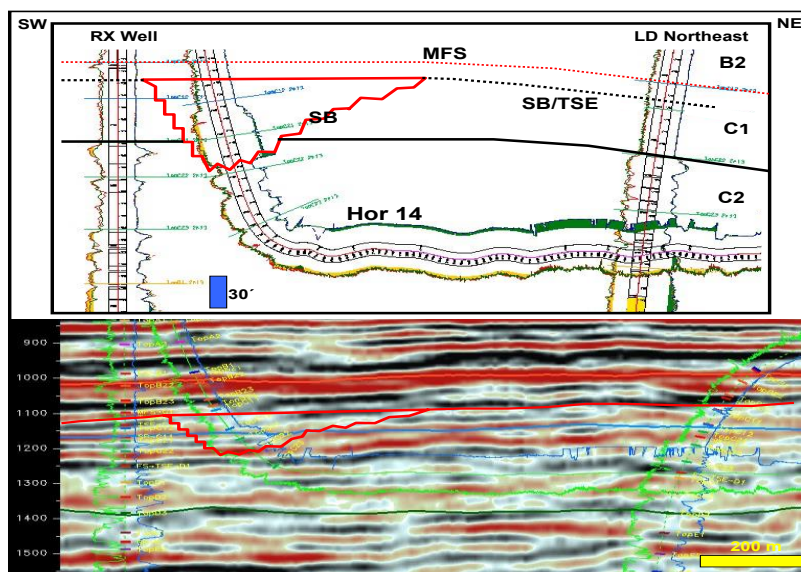
Fig 12: Well cross section and seismic line from cluster SE showing horizontal well Hor 14. In its inclined section, the well cross a thick sandbody (50 feet thick) in C1 unit, which is not in the well RX (200 meters away). The sandbody also is absent in well LD Northeast.
