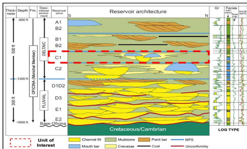
Fig 4: Stratigraphic model modified from [6, 7] with the operational subdivision and the architecture for Lower Oficina Formation (Morichal Member).
