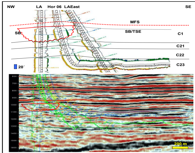
Fig 13: Example in seismic and well cross section for cluster LA, showing wells LA and Horizontal 06 crossing a thick sandbody in operational unit C1. The sandbody is absent 430 meters away in control well LA East.
