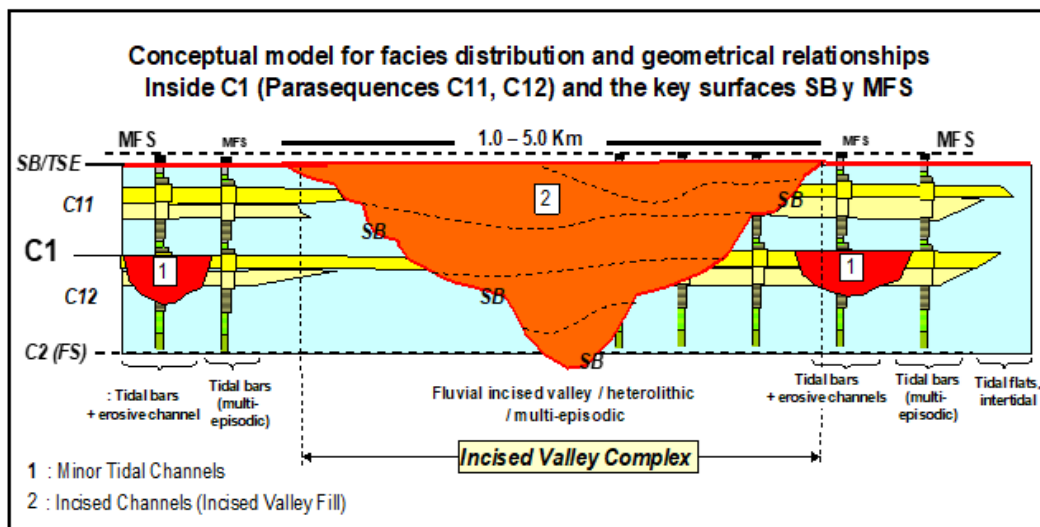
Fig 10: Conceptual model regarding the distribution of facies associations and genetic relationships, to explain the presence of an incised valley system complex in C1.
