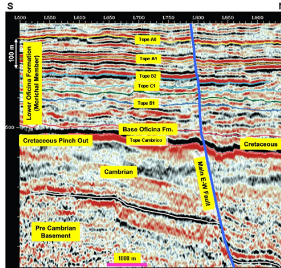
Fig 3: North-south seismic section across the study area showing the stratigraphy and the main interpreted seismic markers, along the operational units defined in the field. The main structural feature is an east-west fault crossing the entire field. Modified from [5].
