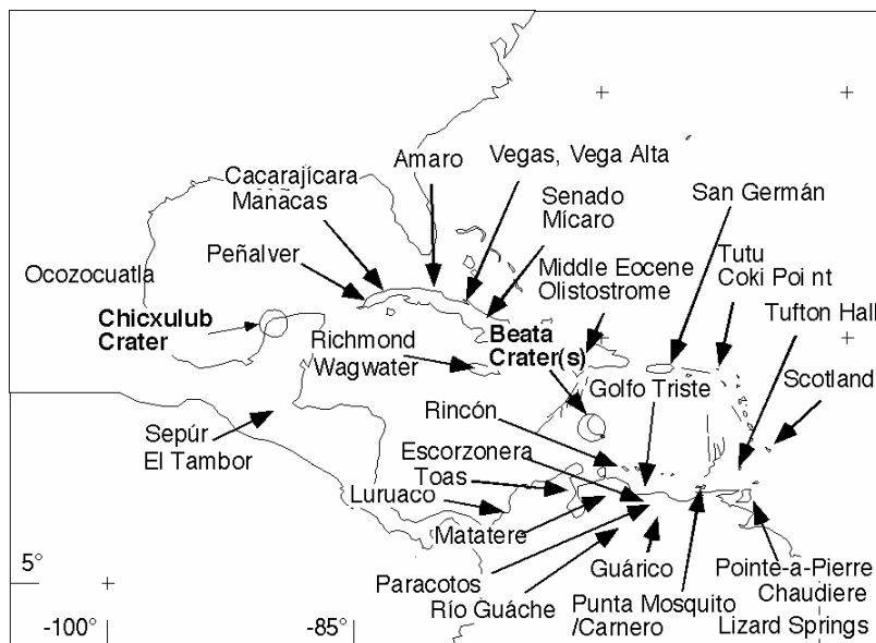
Figure 1. Occurrences of Palaeocene-Middle Eocene flysch/wildflysch deposits and location of the Beata Crater.
