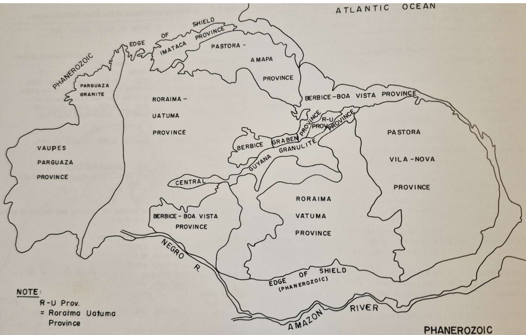
Figure 1.5. Geological provinces (Gibbs, 1987).
