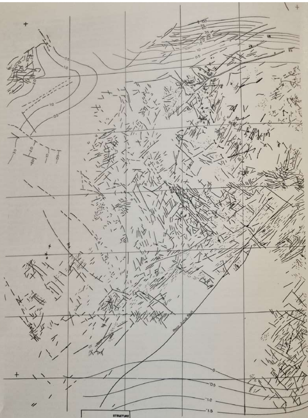
Figure 1.7. Lineament and structure map of the Guiana Shield. Compiled by A. K. Gibbs for this publication.
